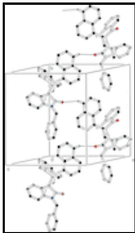
Fig. 3. Molecular packing of the title compound, viewed along the c axis; H-bonds are shown as dashed lines forms a C(12) chain motif in unit cell. For the sake of clarity, H atoms, not involved in hydrogen bonds, have been omitted
