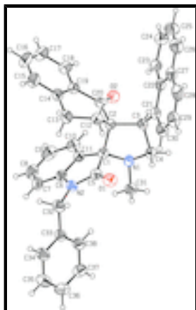
Fig. 1. The molecular structure of the title compound, showing the atom-numbering scheme. Displacement ellipsoids are drawn at the 30% probability level
