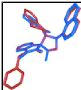
Fig. 2. Superposition of (I) (red) with the similar reported structure of Selvanayagam et al. (2011) (blue).
